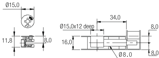
MF 16 for 16mm board
