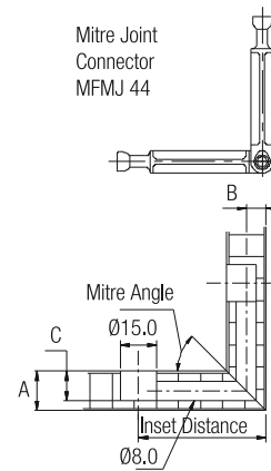
Drilling Diagram for Mitre Joint Connector
