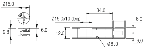
MF 12 for 12mm board
