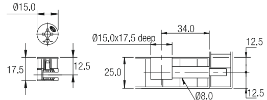
MF 25 for 25mm board
