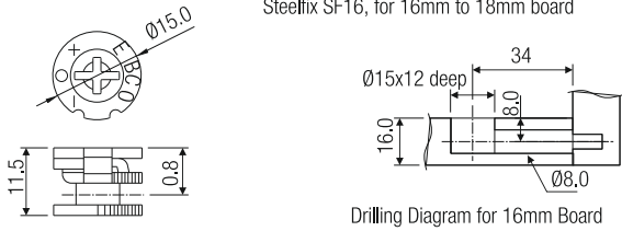
Steelfix SF16, for 16mm to 18mm board
