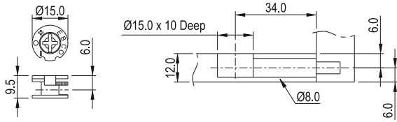
Steelfix Housing 12mm
