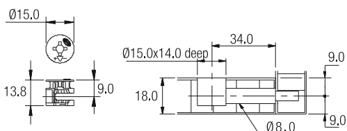
MF 18 for 18mm board
