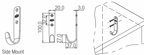
Side Mount
